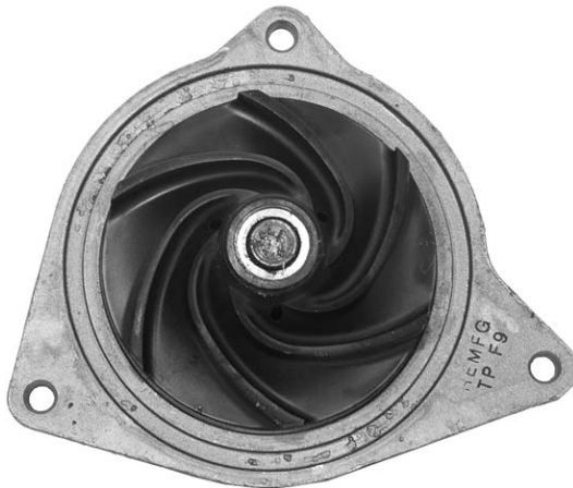
58-541 with 3 mounting holes
