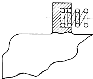
COUNTERBORE DESIGN
