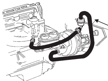
EXAMPLE OF IN-LINE FILTER AND HOSE LOOP
